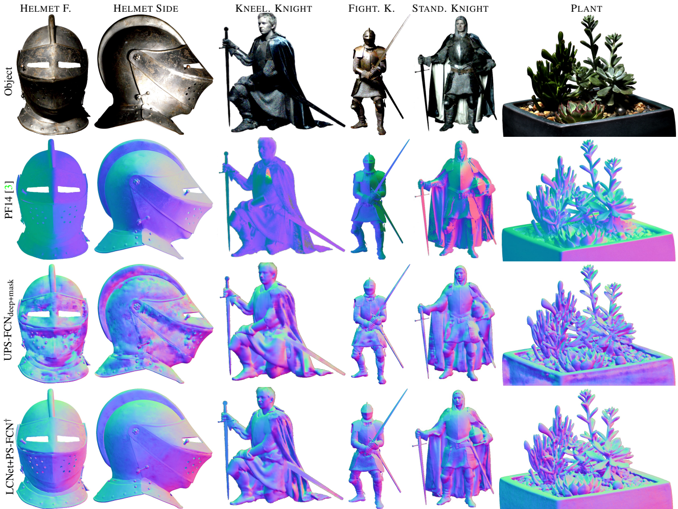
Figure 13. Qualitative results of uncalibrated photometric stereo on Light Stage Data Gallery. Note that although UPS-FCN_{deep+mask} produced good results for the DiLiGenT benchmark, it had difficulty in handling the objects in Light Stage Data Gallery and Gourd&Apple Dataset. This is because the image sizes of these two datasets are considerably larger (e.g., PLANT: 1200 \times 850 , APPLE: 650 \times 700 ), compared with the DiLiGenT benchmark (e.g., READING: 200 \times 220 ). Single-stage methods estimate surface normals for each patch based solely on the observations of that patch and thus tend to produce noisy estimation when the image size is large. In contrast, the proposed two-stage method first estimates the global directional lightings using the whole image and then estimate the surface normals based on the lighting and observations. This result reiterates the advantage of our two-stage method.
